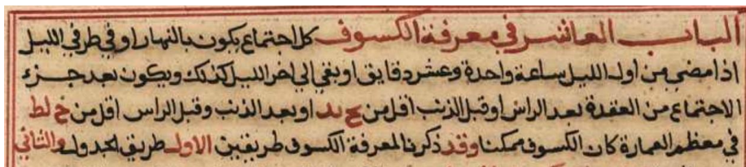
Figure 1. Zij-i Sultānī text: conditions for the occurrence of a solar eclipse based on the location of the conjunction
