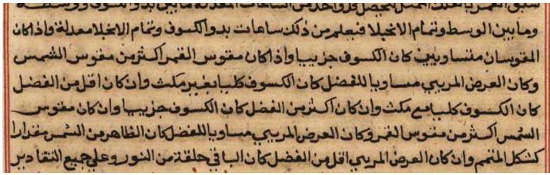
Figure 4. Zīj-i Sultānī text: parameters of eclipse types
