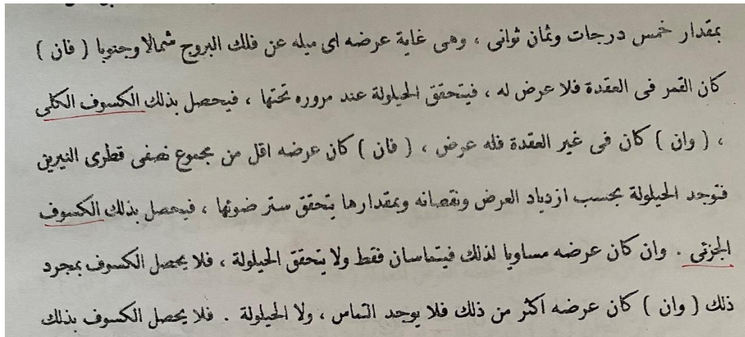
Figure 6. Text of Sullam al-Nayyirain
