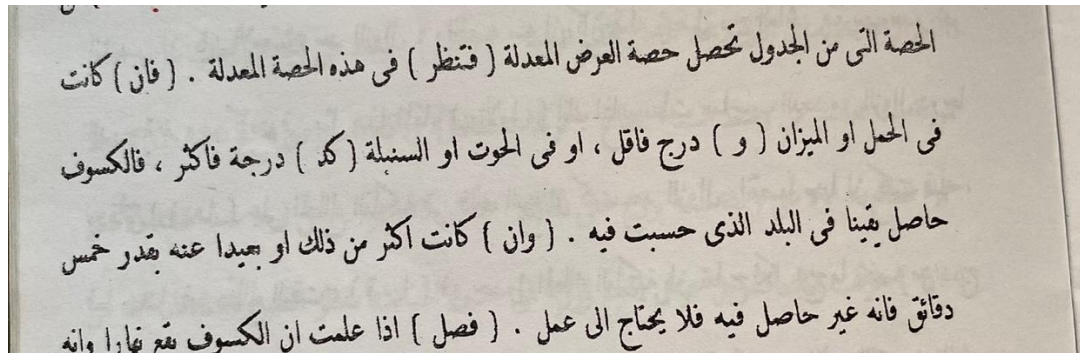
Figure 5. Text of Sullam al-Nayyirain
